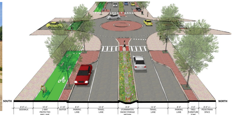
Cross-Section - West State Street between 1st and 11th Streets Olean, NY
